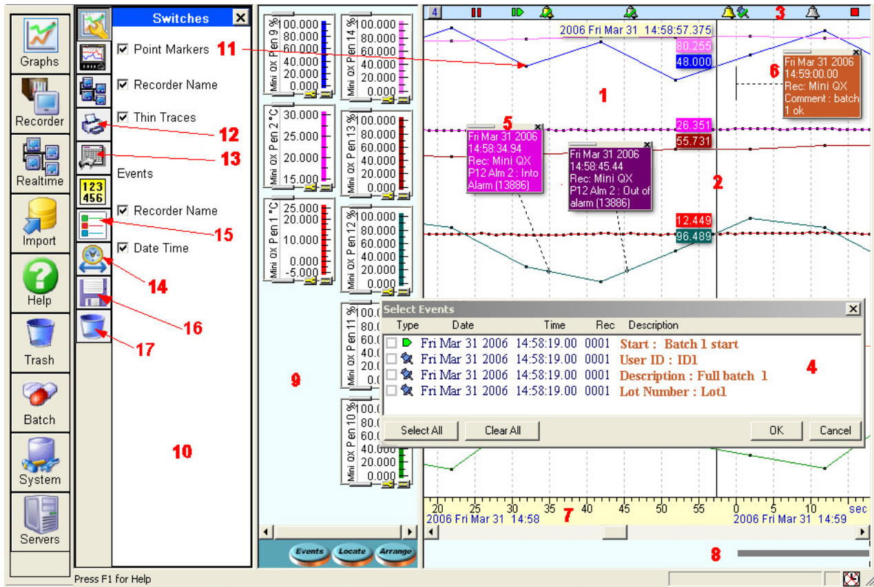
Figure 1.2 User Interface
