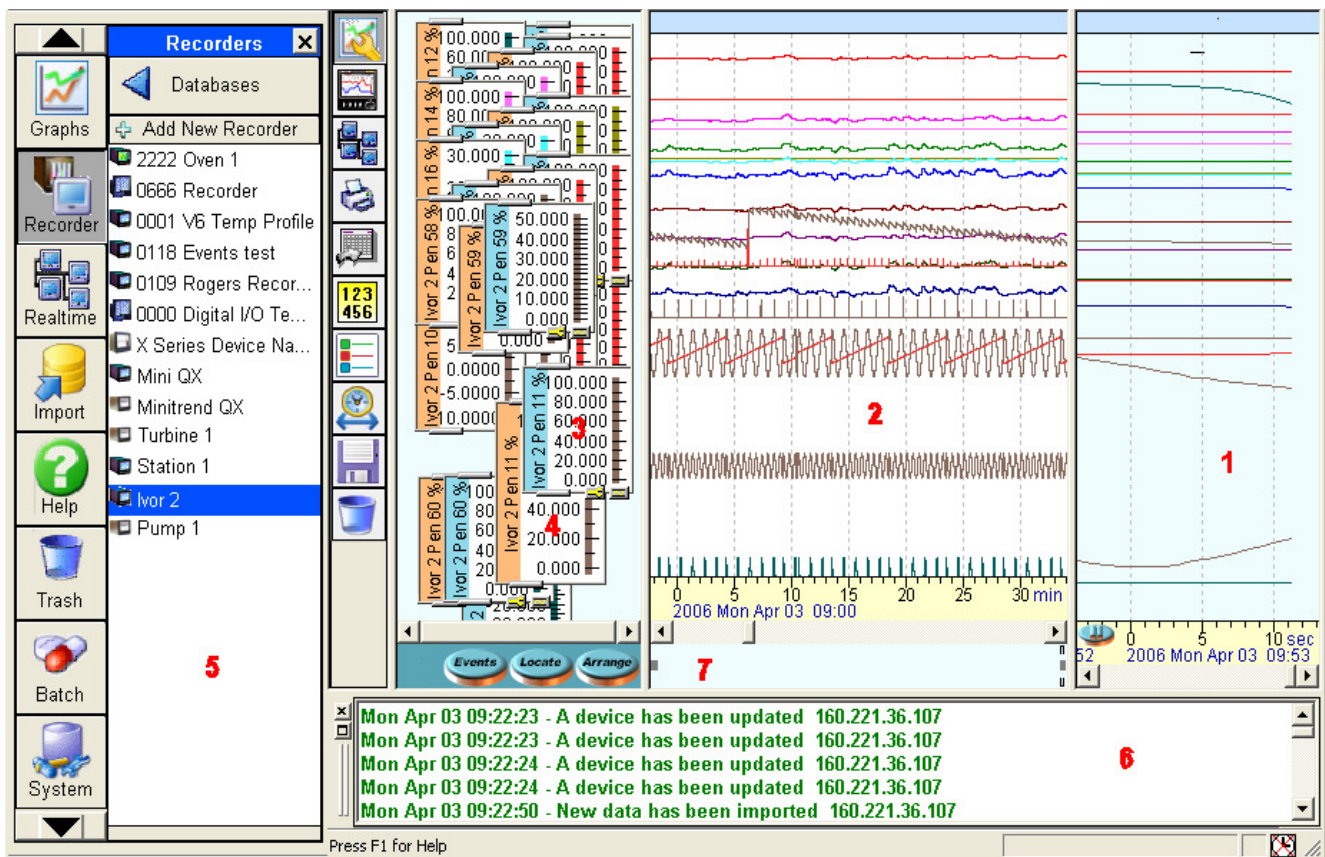
Figure 1.4 Interface Areas
