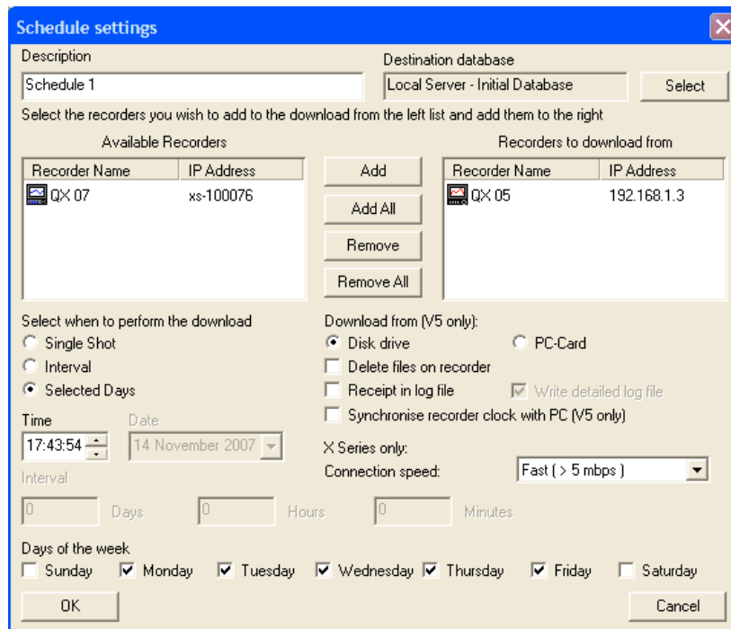
Figure 1.7 FTP Scheduler
