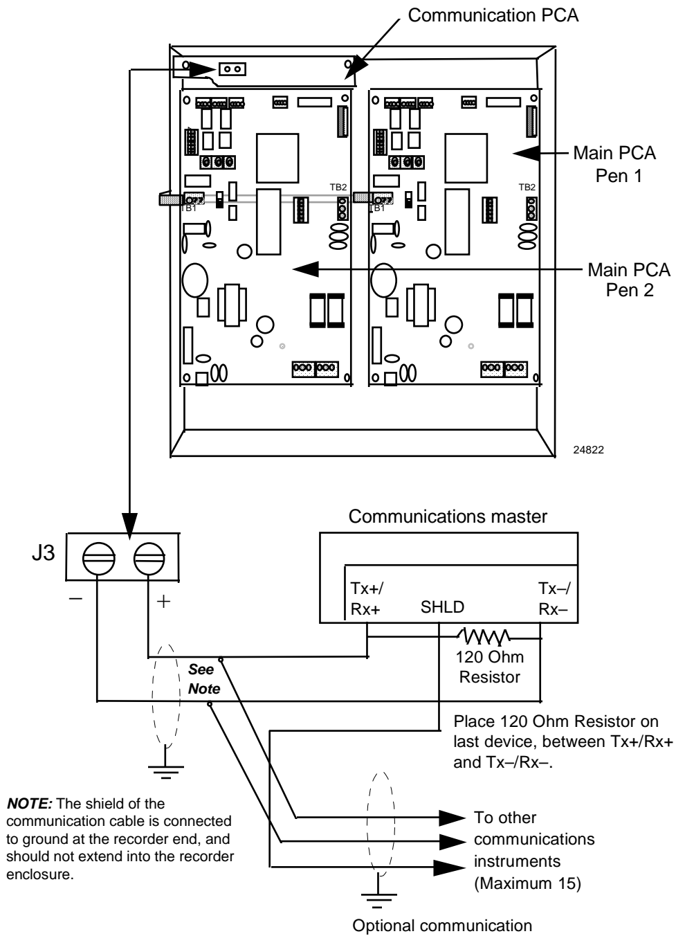
Figure 2-13 Communication Wiring
