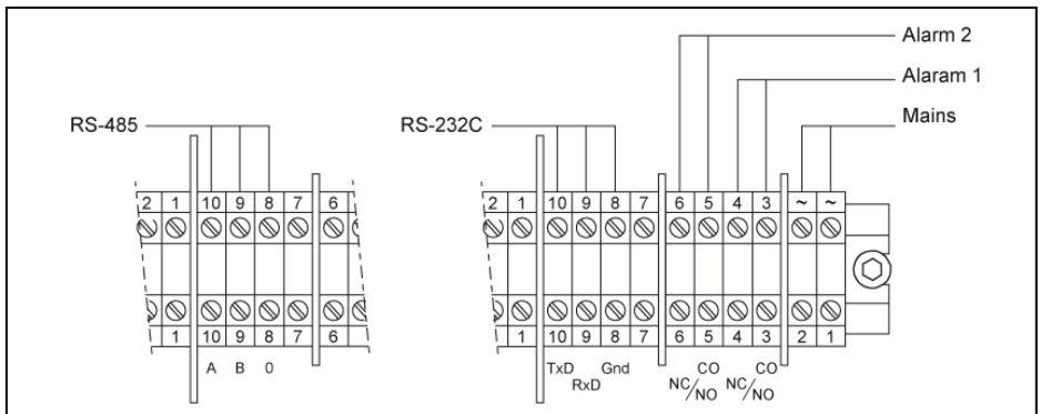
Figure 8 RS-232C / RS-485 connections
