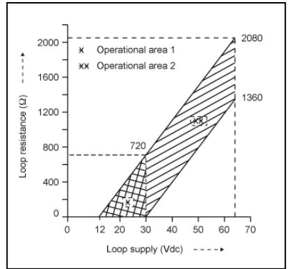
Figure 7 Selecting the external loop resistor
