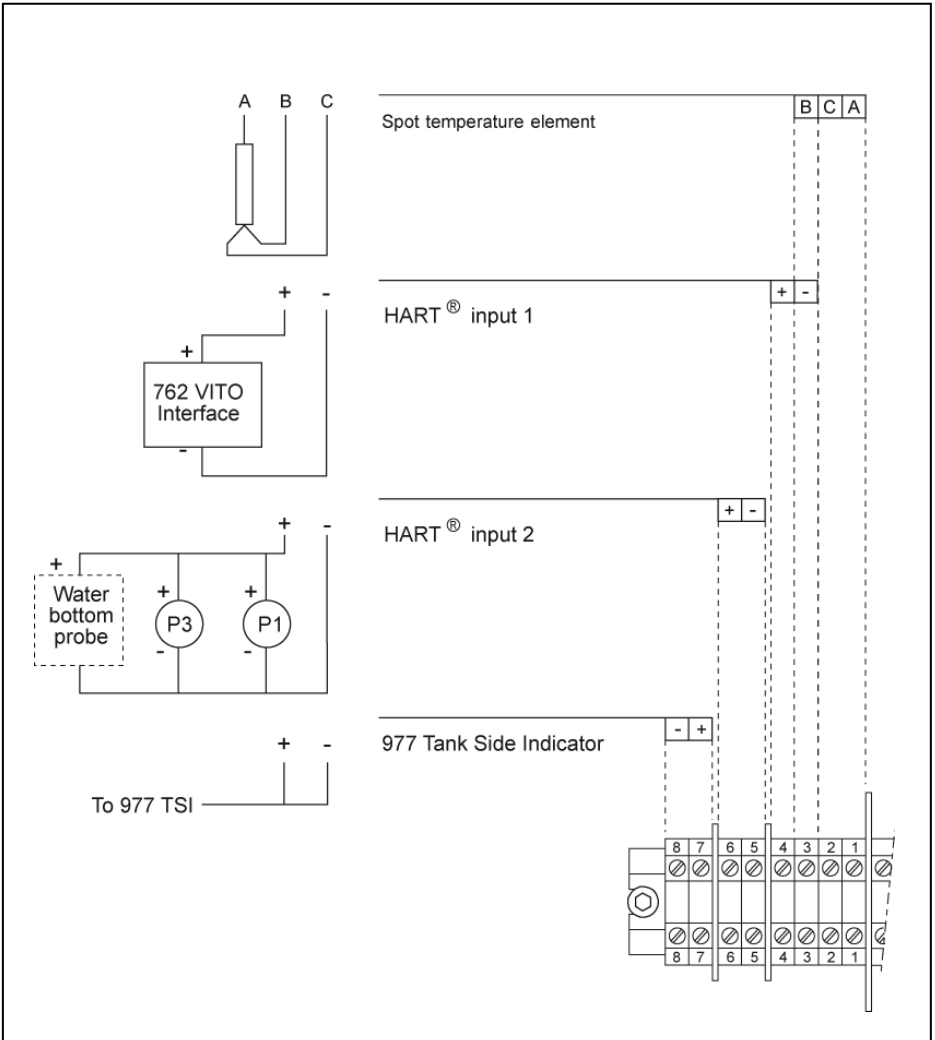
Figure 9 Intrinsically safe connections with HCU option board
