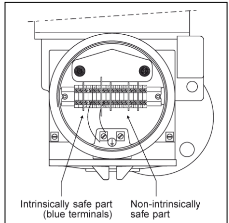
Figure 5 Terminal compartment 854 XTG
