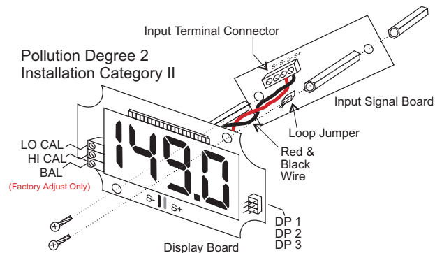
Figure 1. Assembly
