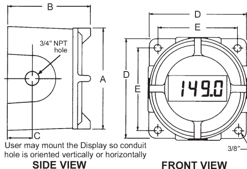
Figure 3. Dimensions and Mounting Information
