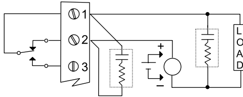
Figure 27. AC and DC Loads Protection
