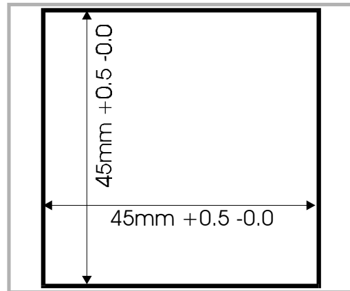
Figure 1-1 Cut-out Dimensions
