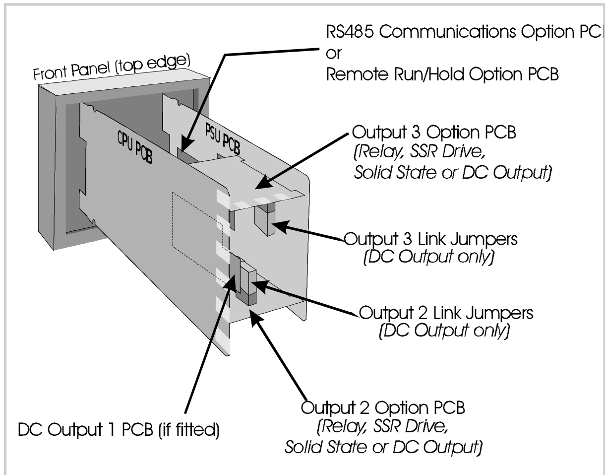
Figure 2-1 PCB Positions
