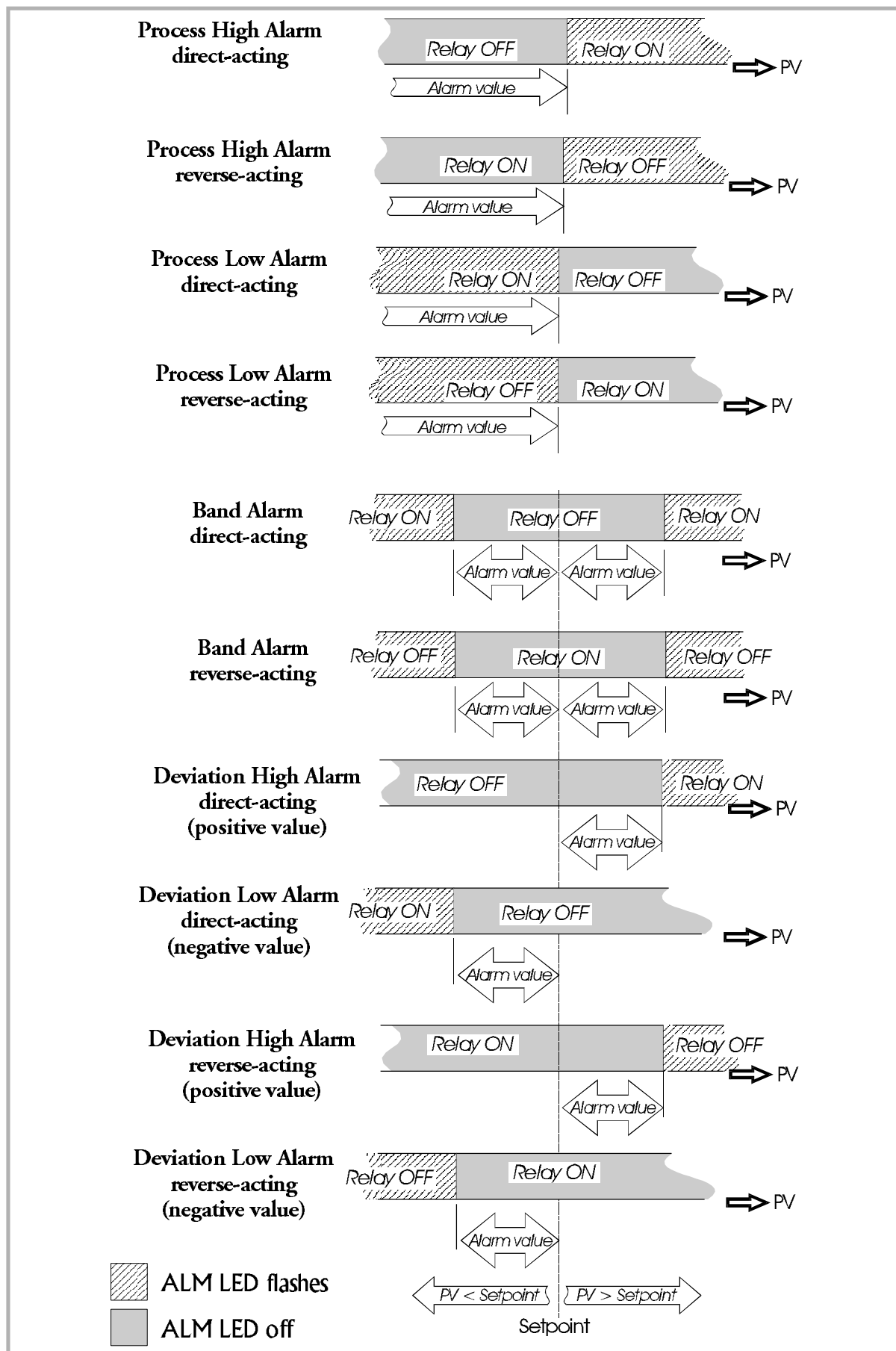
Figure 3-2 Alarm Operation
