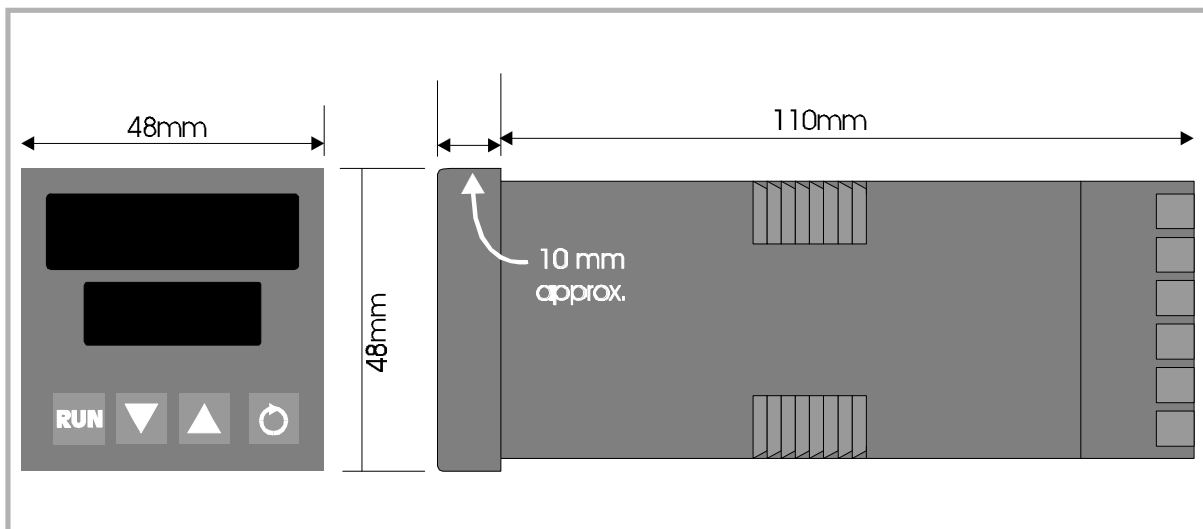
Figure 1-2 Main Dimensions
