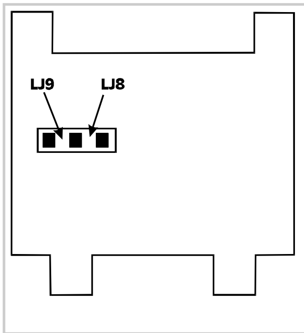
Figure 2-6 DC Output Option PCB (Output 2/Output 3)
