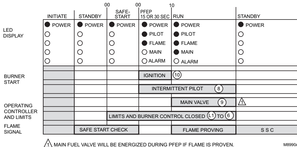
Fig. 12. RM7890D sequence.
