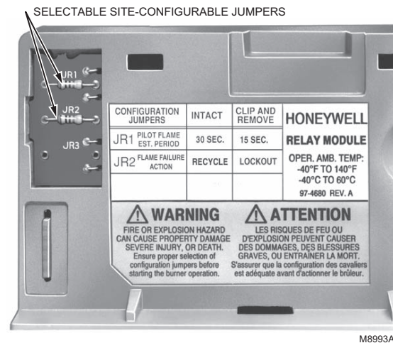
Fig. 15. Selectable site-configurable jumpers (RM7890).
