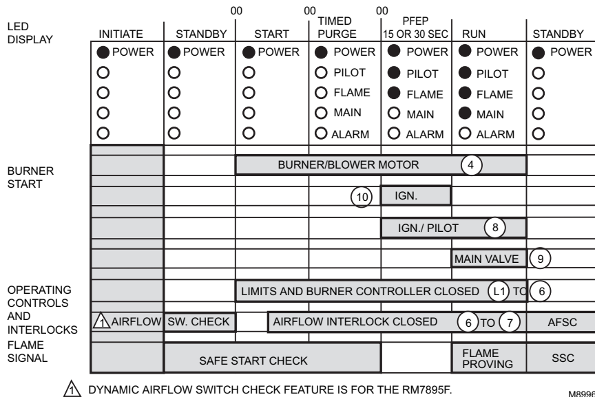
Fig. 13. RM7895E,F sequence.
