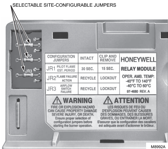
Fig. 16. Selectable site-configurable jumpers (RM7895).
