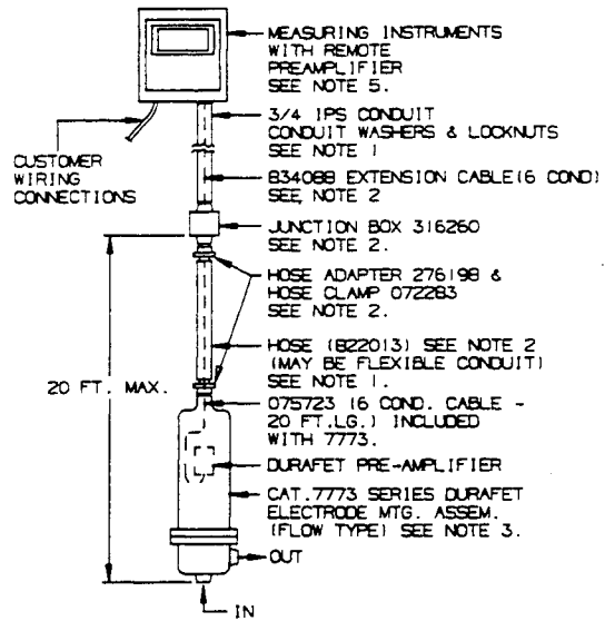
FIG. 2 PRE-AMP TO MEASURING INSTRUMENT SEPARATION GREATER THEN 20 FT.
