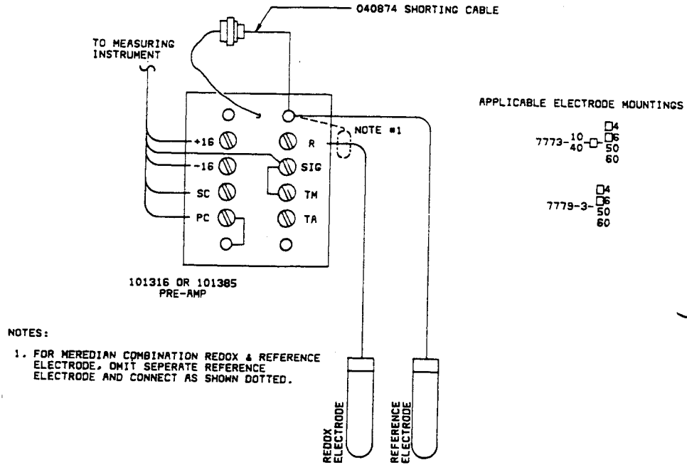
Figure 3-14 Drawing No. A-ID-081606-15 - ORP Connections for 7773-10, 40 and 7779-3 Electrode Mounting Assembly with Preamp
