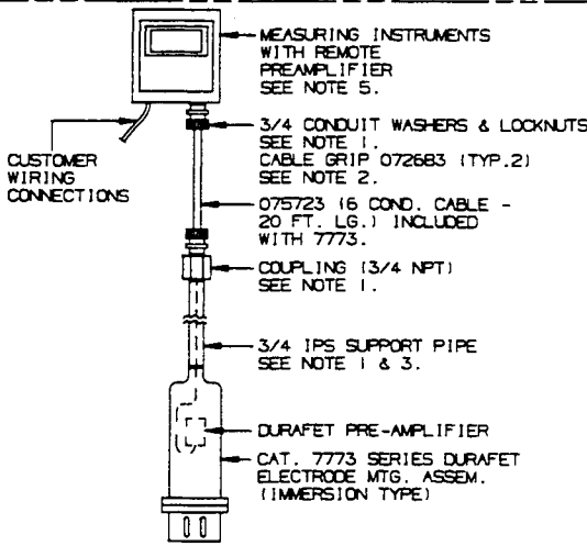
FIG. 3 PRE-AMP TO MEASURING INSTRUMENT SEPARATION 20 FT. OR LESS
